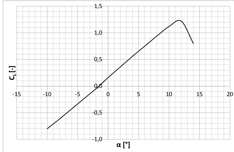
Figur 4: Liftkurve. Her vist for NACA 23012 profil.
