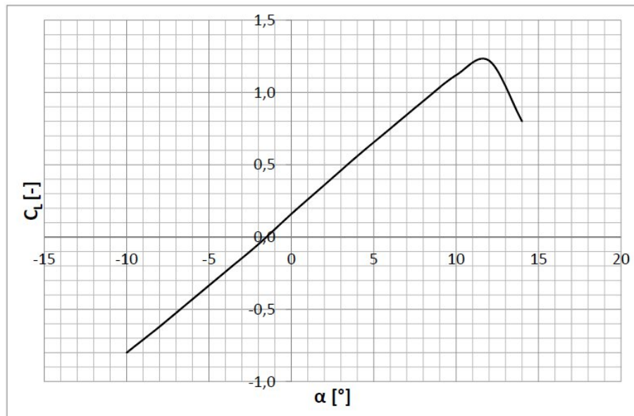
Figur 4: Liftkurve. Her vist for NACA 23012 profil.
